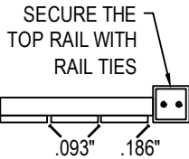
DETAIL A PICKET SPACING
