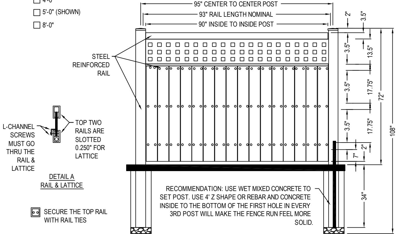
FRONT ELEVATION
