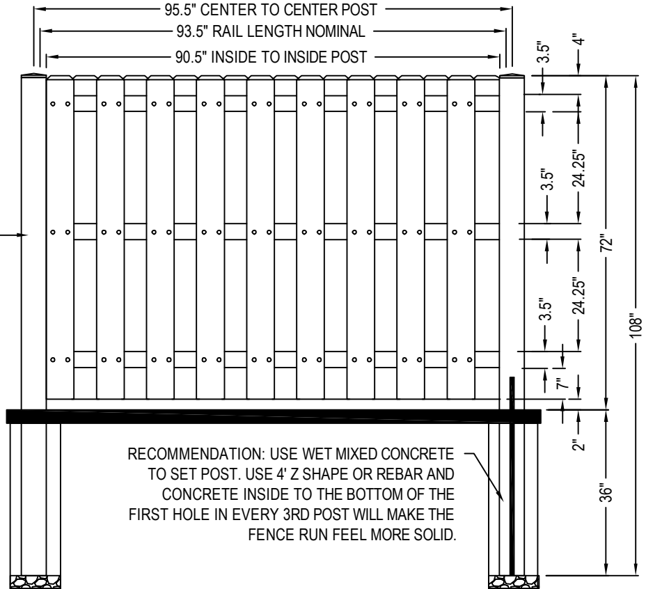
FRONT ELEVATION
