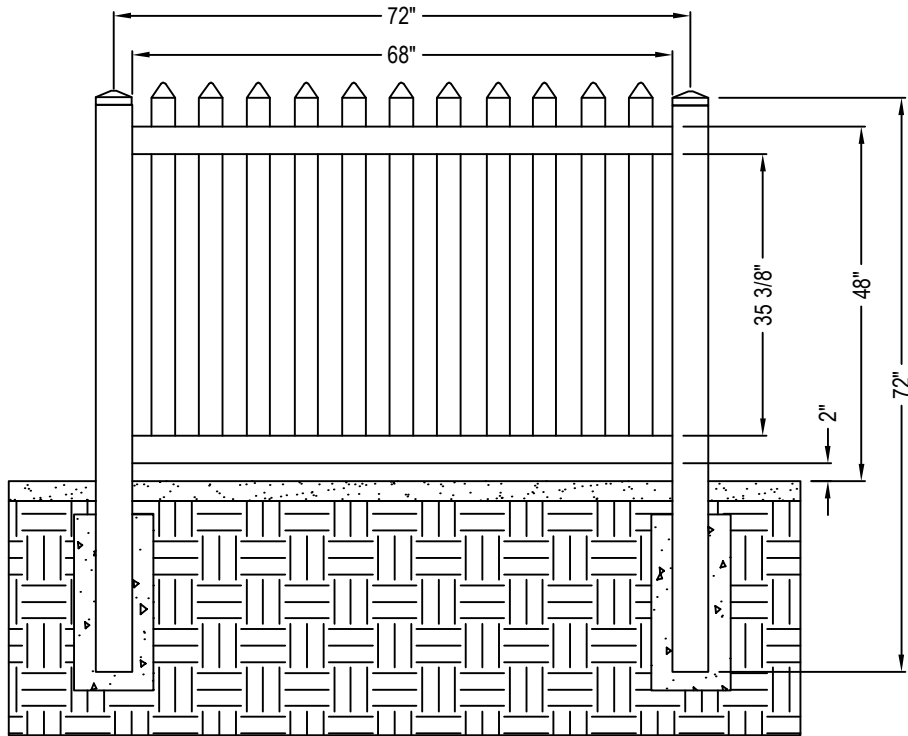
FRONT ELEVATION
