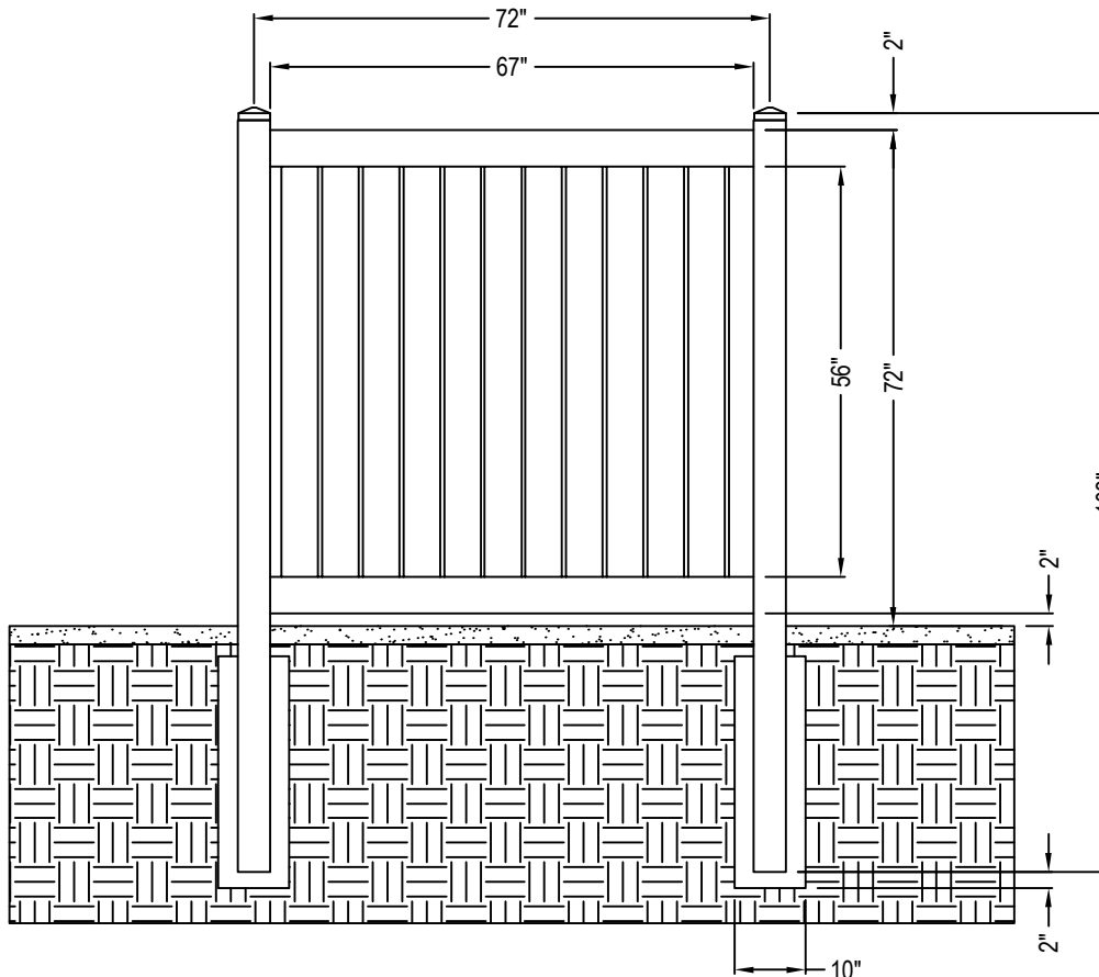
FRONT ELEVATION
