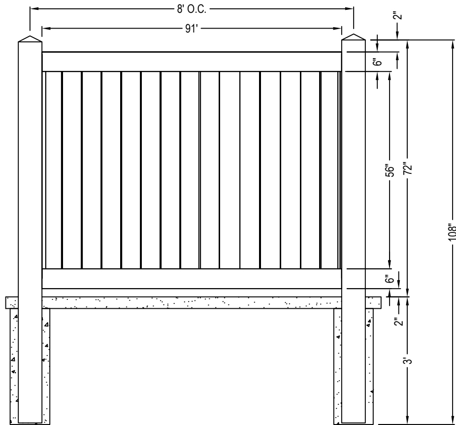
FRONT ELEVATION
