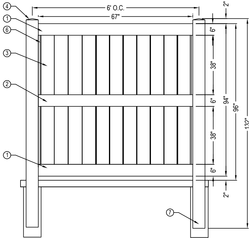
FRONT ELEVATION
